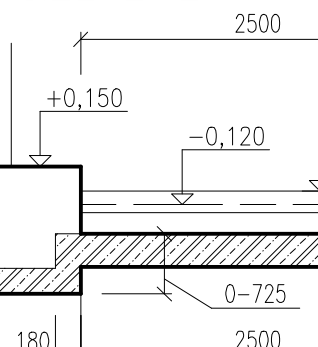
REZ E-E
